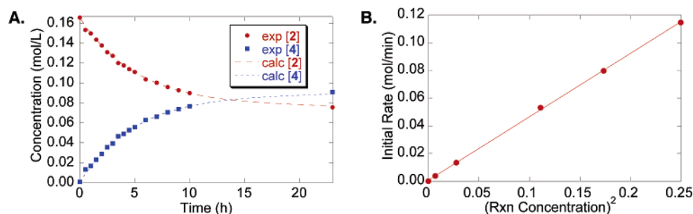
Figure 1. (A) Representative time-course for \text{Al}_2(\text{NMe}_2)_6 -catalyzed transamidation between 2 and 3 (eq 4). The calculated curve fits reflect a nonlinear least-squares fit of the data to an equation associated with a bimolecular approach to equilibrium ( [\text{A}]_t = [\text{A}]_{\infty} + ([\text{A}]_0 - [\text{A}]_{\infty}) e^{-kt} , k = k_1 + k_{-1} ). Conditions: [\text{Al}_2(\text{NMe}_2)_6] = 4.2 \text{ mM} , [\text{carboxamide}] = 0.17 \text{ M} , [\text{amine}] = 0.17 \text{ M} , 5 \text{ mL} toluene, 90 \text{ }^\circ\text{C} . (B) Kinetic plot demonstrating a linear correlation between the rate and the square of the “reaction concentration” (linear least-squares curve fit). The “reaction concentration” (defined in the text) is arbitrarily assigned as the initial carboxamide concentration.
