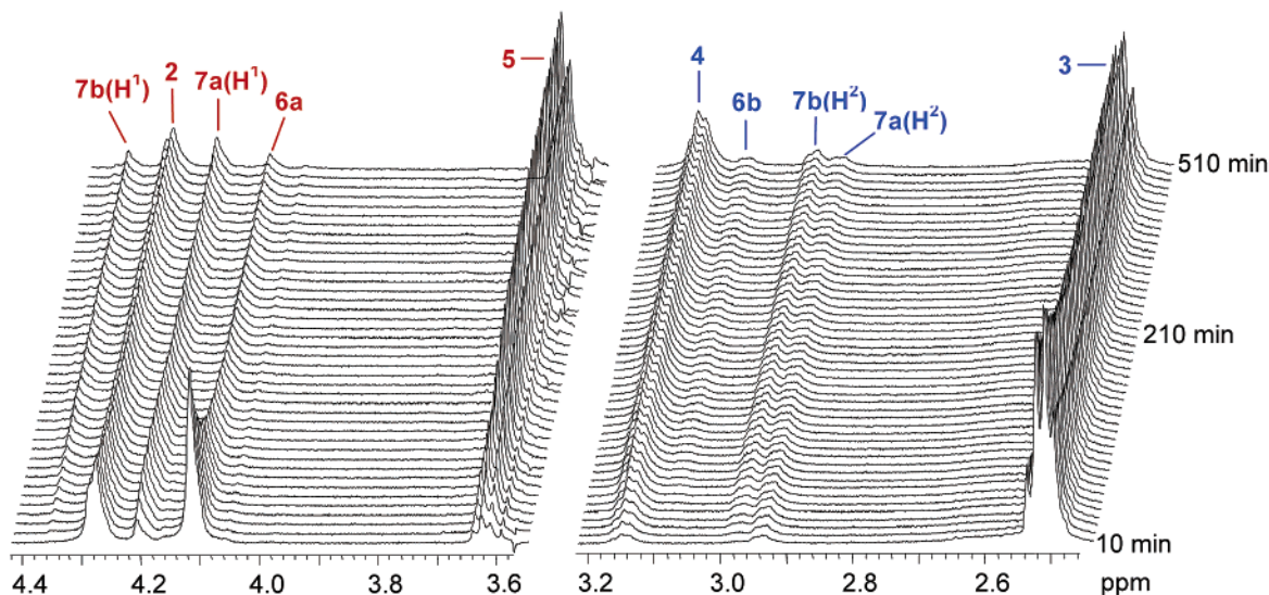
Figure 5. ^1\text{H} NMR spectral time-course for \text{Al}^{\text{III}} -catalyzed transamidation reaction between 2 and 3 (90 °C in toluene- d_8 ). Data were collected until the reaction reached equilibrium. The first spectrum was acquired 10 min after mixing, and additional spectra were acquired at 5-min intervals. The spectra display the diagnostic resonances of the \text{CH}_2 group adjacent to nitrogen in the amine and carboxamide reagents and products. The internal standard peak at 3.41 ppm (1,3,5-trimethoxybenzene) has been removed for clarity. Initial conditions: [\text{Al}_2(\text{NMe}_2)_6] = 0.083 \text{ M} , [\mathbf{2}] = [\mathbf{3}] = 0.17 \text{ M} .
