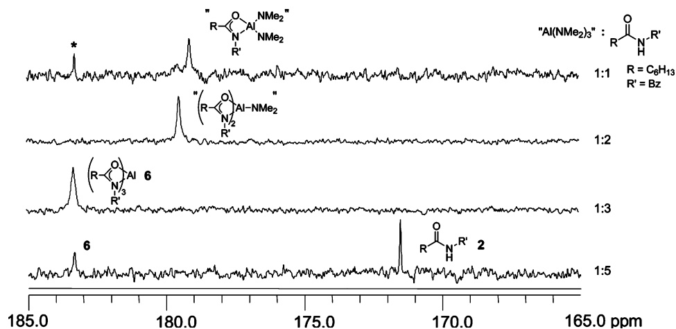
Figure 4. ^{13}\text{C} NMR spectra monitoring the changes that occur in the carbonyl region upon addition of N -benzylcarboxamide 2 to a solution of \text{Al}_2(\text{NMe}_2)_6 in toluene- d_8 . The \text{Al}^{\text{III}} :carboxamide ratio present in each solution is indicated on the right-hand side of the spectra. [Note: ^1\text{H} NMR data (Figure S3) reveal that the peak labeled with an asterisk in spectrum for 2:Al = 1:1 does not arise from the same complex as that present at 2:Al ratios \geq 3:1 .]
