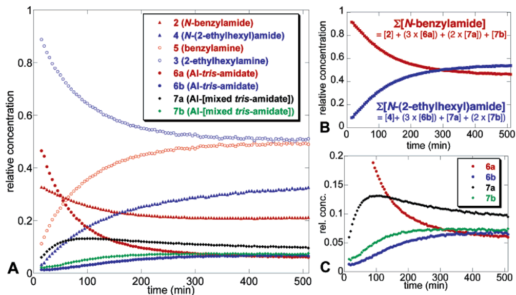
Figure 6. (A) Reaction time-course of the \text{Al}^{\text{III}} -catalyzed transamidation between 2 and 3 in toluene- d_8 at 90 °C. The concentrations of the species were determined by ^1\text{H} NMR spectroscopy, sampling every 5 min, with the initial time point at 10 min. Concentrations are plotted for amines 3 and 5 , carboxamides 2 and 4 , and the aluminum amidates 6a , 6b , 7a , and 7b . The concentrations of mixed \text{Al}^{\text{III}} -amidates 7a and 7b were determined from the weighted average of the two resonances associated with each amidate. Initial conditions: [\text{Al}_2(\text{NMe}_2)_6] = 0.083 \text{ M} , [\mathbf{2}] = [\mathbf{3}] = 0.17 \text{ M} . (B) Total carboxamide concentration present in the reaction, accounting for both free carboxamides and \text{Al}^{\text{III}} -coordinated amidates. (C) Expansion of the time-course data revealing the \text{Al}^{\text{III}} -amidate speciation during the reaction.
