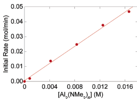
Figure 2. Dependence of the initial rate on catalyst concentration for the transamidation of carboxamide 2 with amine 3 . Initial rates, derived from monitoring the first 5% conversion, were determined by sampling [ 2 ] every 2 min. Conditions: [ 2 ] = [ 3 ] = 0.17 M, 5 mL toluene, 90 °C.
