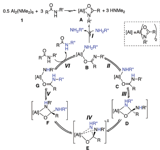
Scheme 1. Proposed Mechanism for Al III -Catalyzed Transamidation
